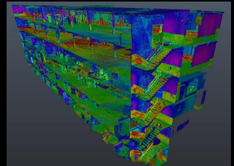
360° Building Scanning
